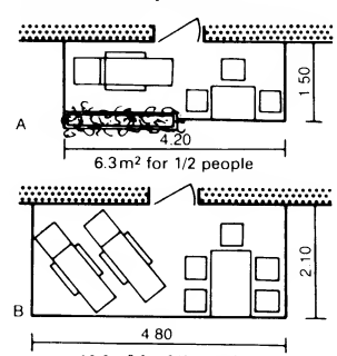
⑭ Balcony layouts
